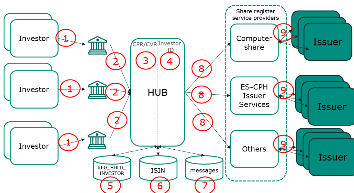
Figure 1: High-level structure of Name Registration service
