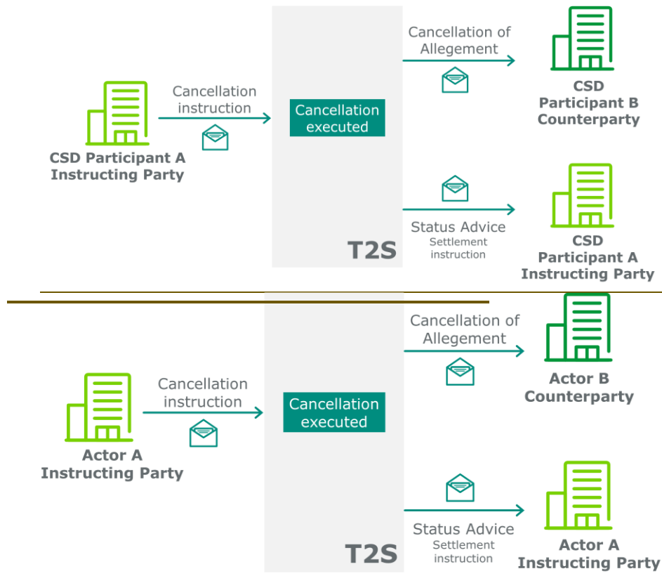
Figure 12 - Scenario for sending a cancellation of the allegement message.
