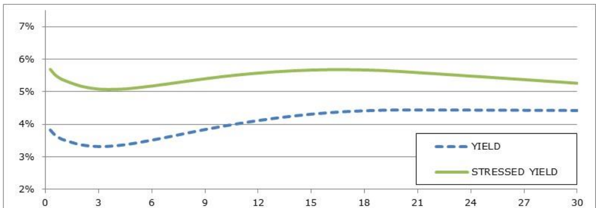
Figure 5: Flattening Scenario (example)
