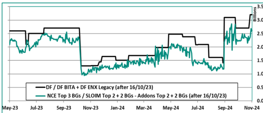
Figure 2 – BITA & LEGACY Equity, Eq. Derivatives and Commodities Derivatives: Historical trend (worst case scenario)
