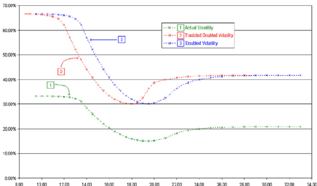
Figure 1 Sticky delta approach with doubled volatility
