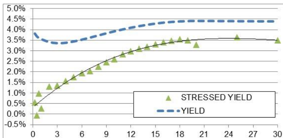
Figure 2: Historical Yield Decrease Scenario (example)
